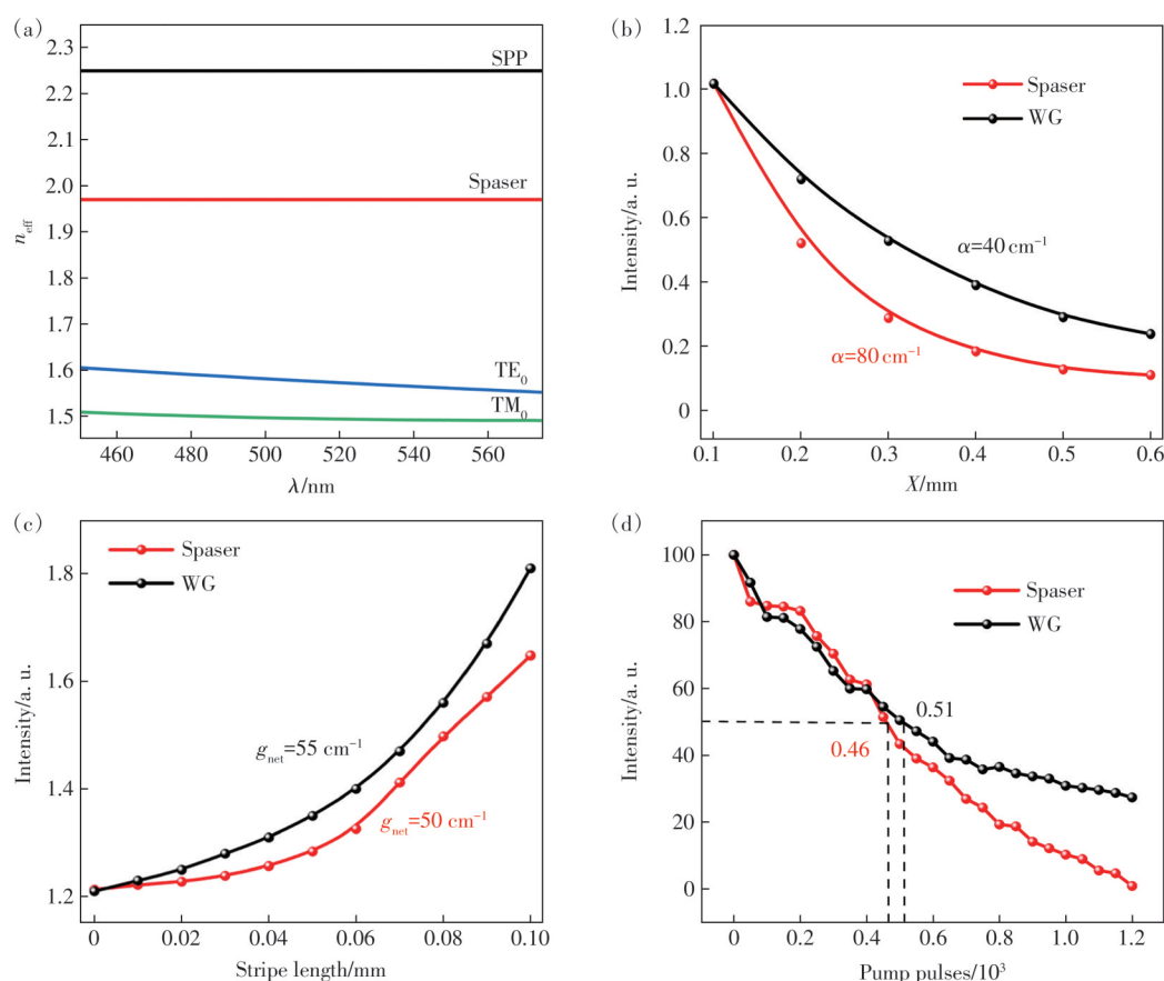
图4 (a)模拟的WG和Spaser样品的模式色散关系;(b)通过SES方法得出的发射强度与未受泵浦作用的传播距离 X 的关系;(c)发射强度随泵浦条长的变化关系;(d)样品在恒定能量密度( \sim P_{\text{th}} )泵浦下输出光强随泵浦脉冲数量的变化 Fig.4 (a) The simulated mode dispersion relation of the WG and Spaser samples. (b) Emission intensity as a function of unpumped propagation distance X , obtained via SES method. (c) Emission intensity versus pumped stripe length L , obtained via VSL method. (d) Output intensity dependence on the number of pump pulses under a constant pump fluence ( \sim P_{\text{th}} )
